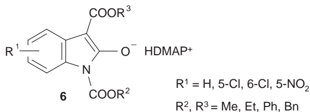
Figure 2. 4-Dimethylaminopyridinium (DMAP) salts of oxindole-1,3-dicarboxylates.
