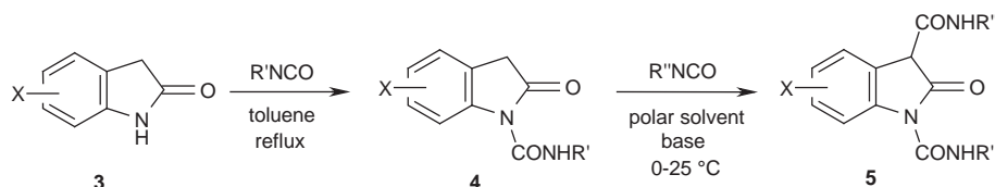
Scheme 1. Literature procedures for the preparation of oxindole-1-carboxamides and oxindole-1,3-dicarboxamides.
